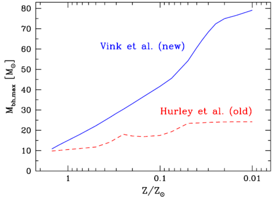
Belczynski et al. 2010
