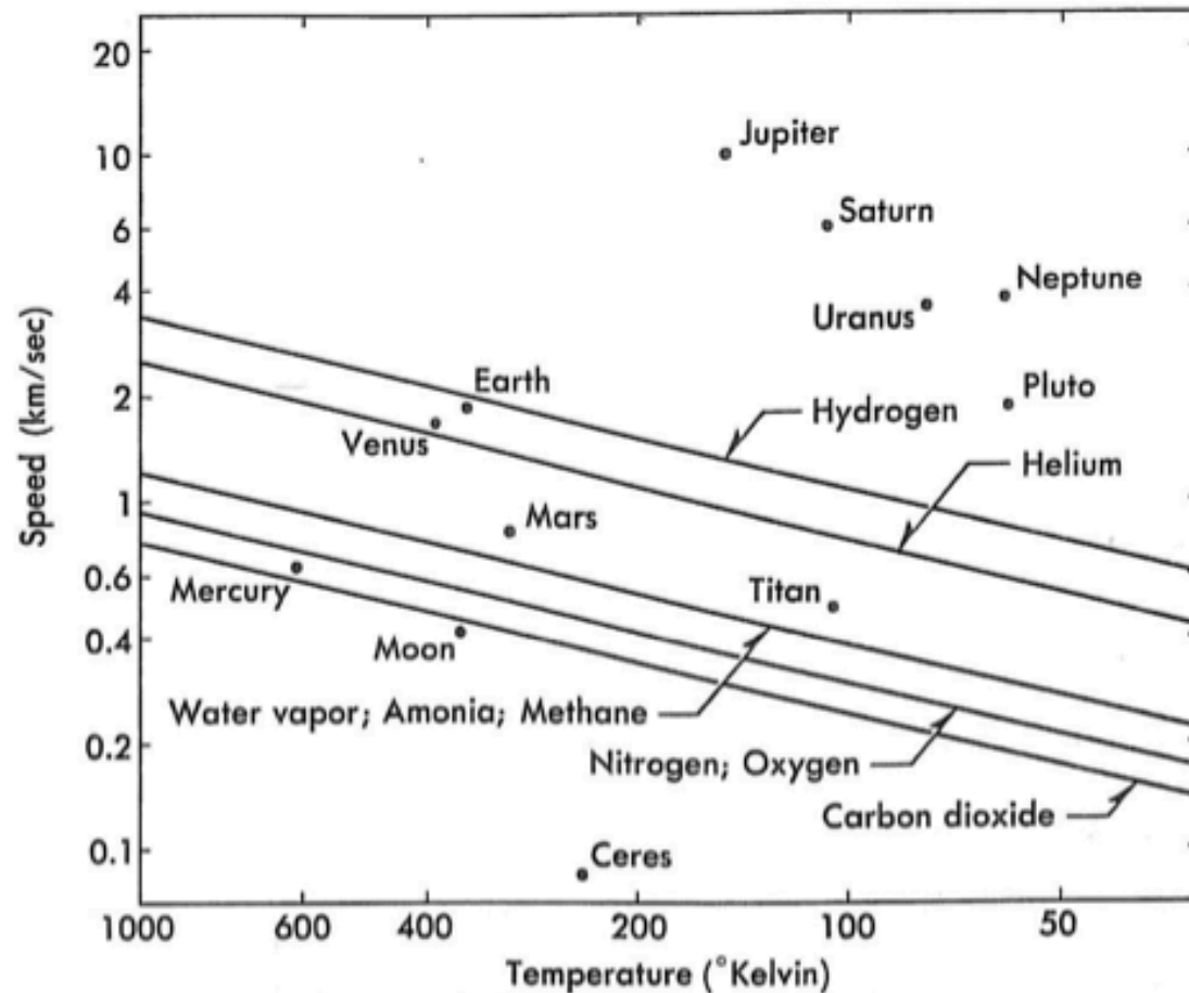
11-2 Molecular speeds of common gases at various temperatures.
