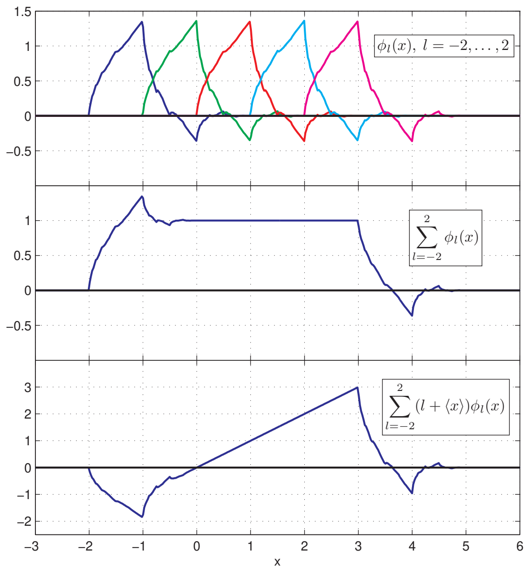
Daubechies-2 Wavelets
