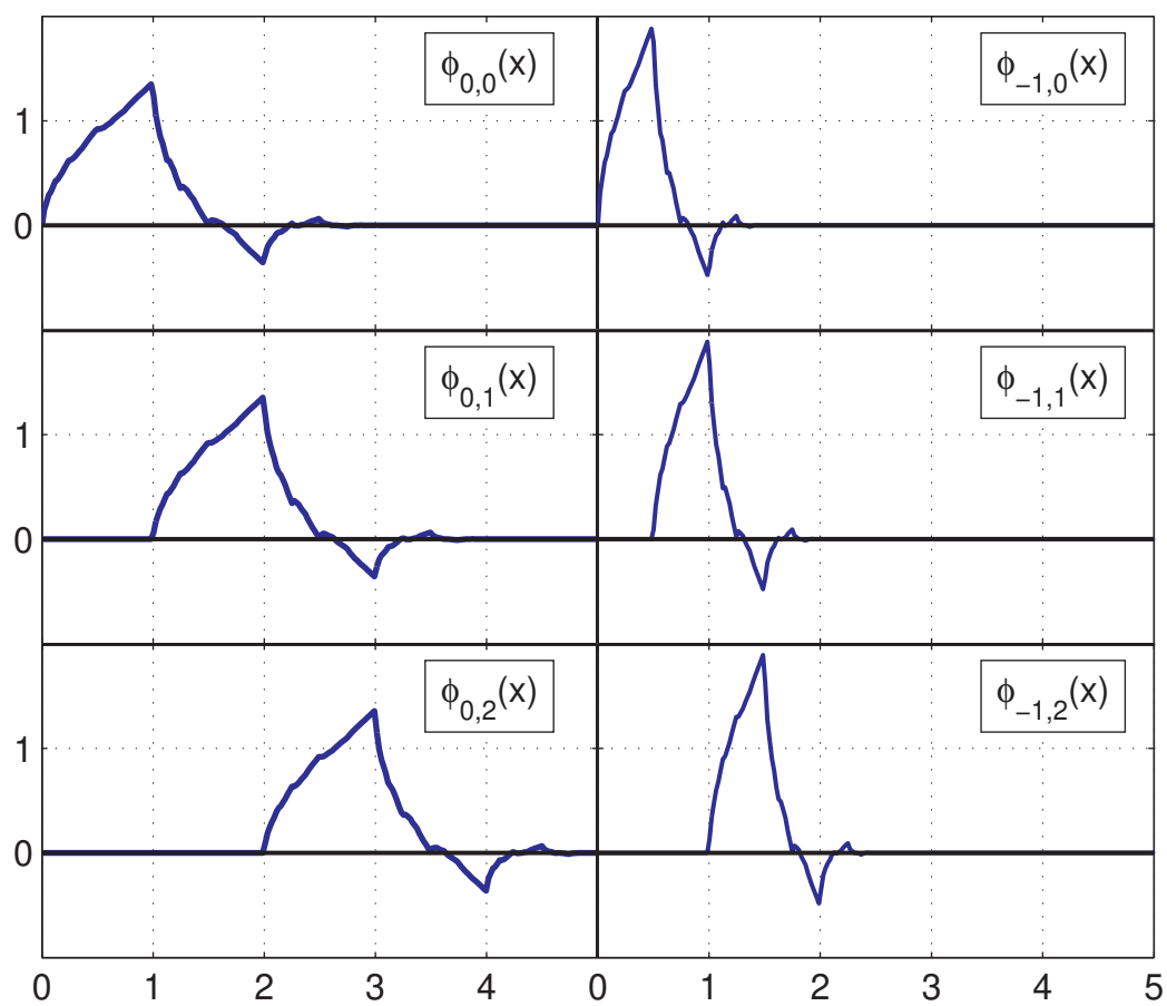
Translations and Dilations – \phi_{j,l}(x)
