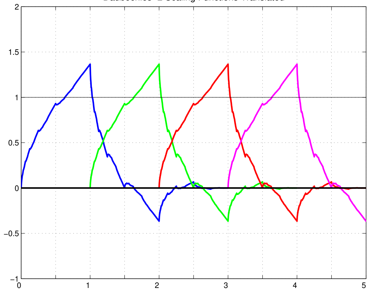
Daubechies-2 Scaling Functions Translated
