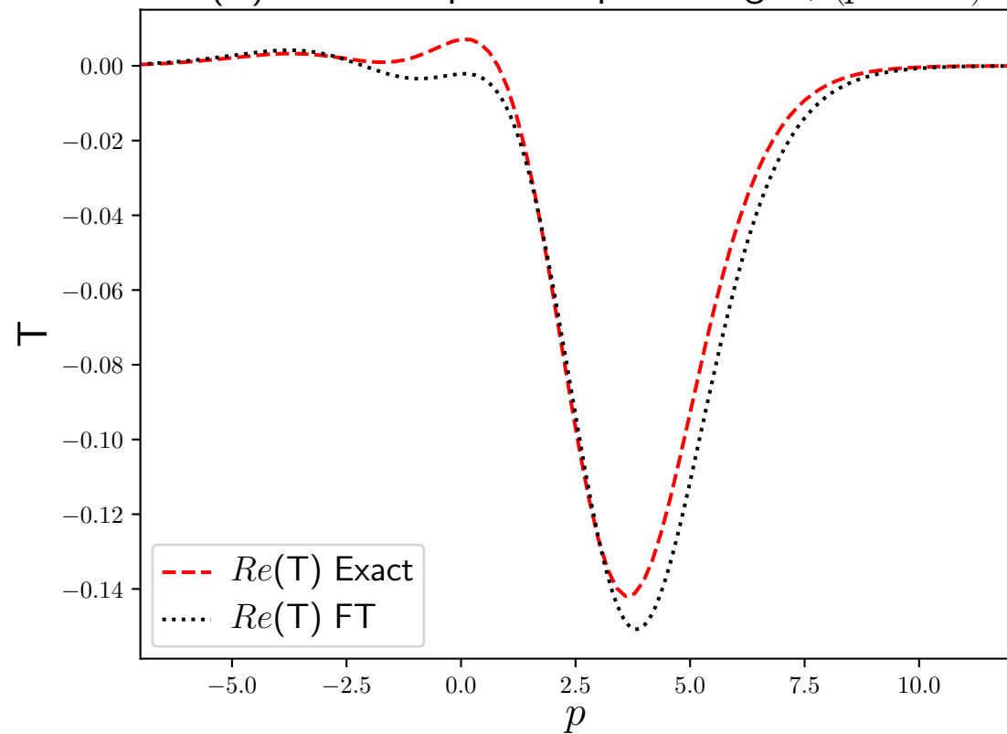
Re(T) exact compared to path integral, ( p = 2.5 )
