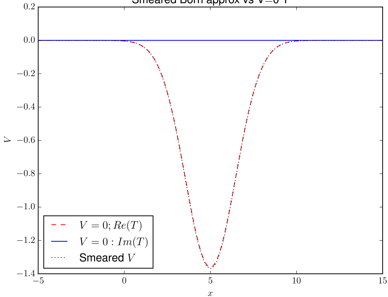
Smeared Born approx vs V=0 T
