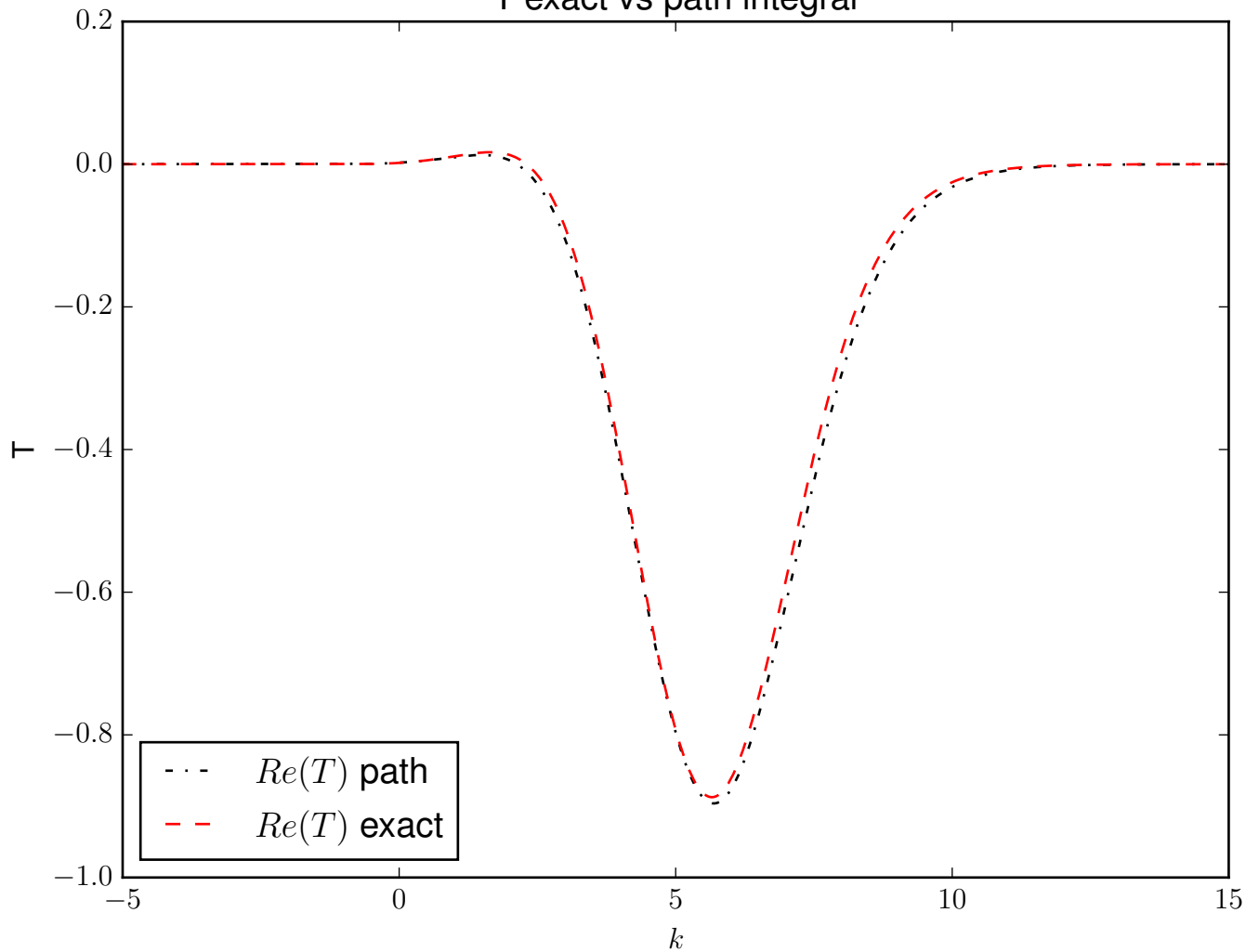
T exact vs path integral
