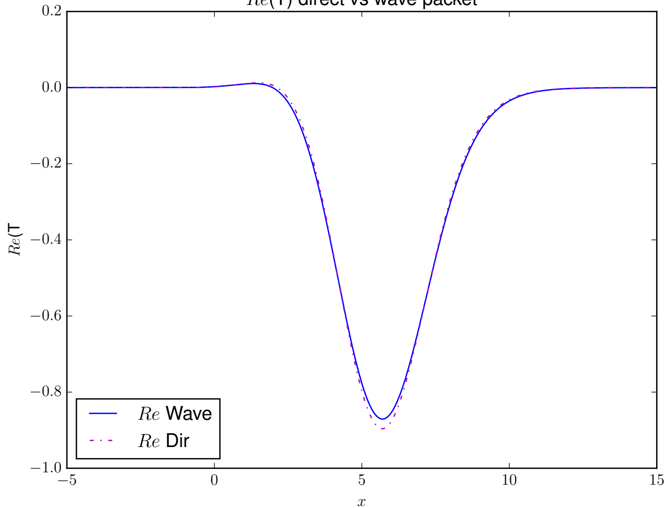
Re(T) direct vs wave packet
