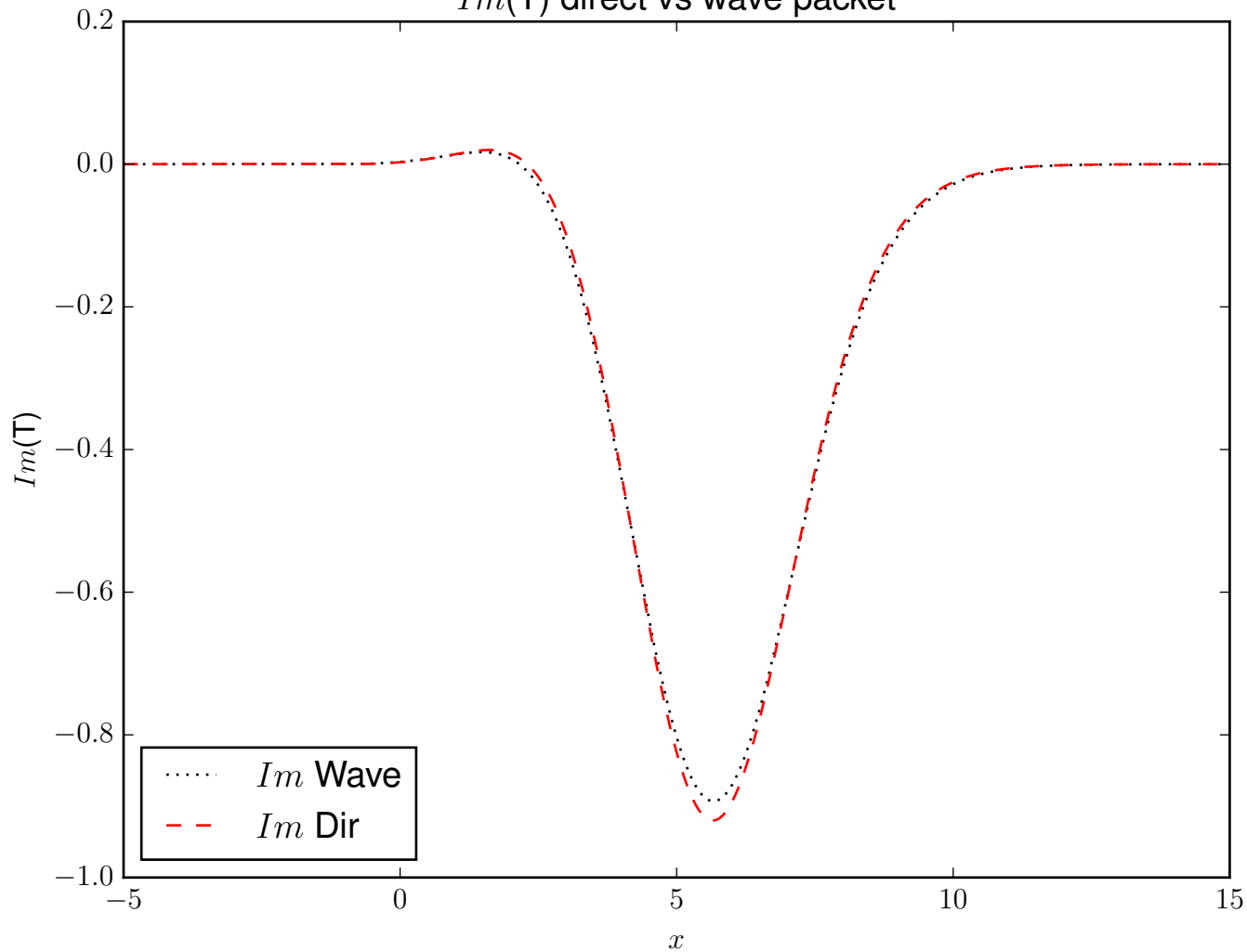
Im(T) direct vs wave packet
