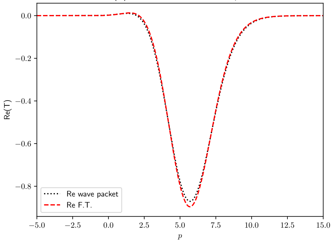
Re (T) Fourier transform vs wave packet
