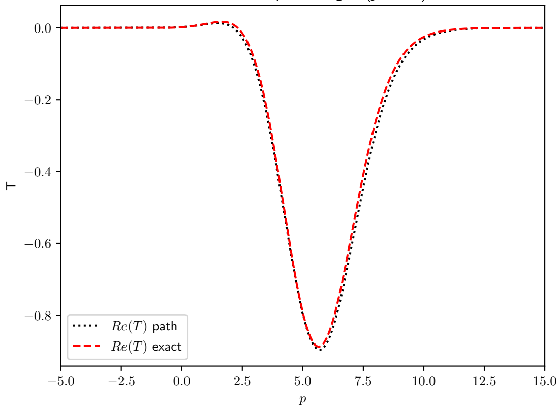
Re T exact vs path integral ( p = 5.0 )
