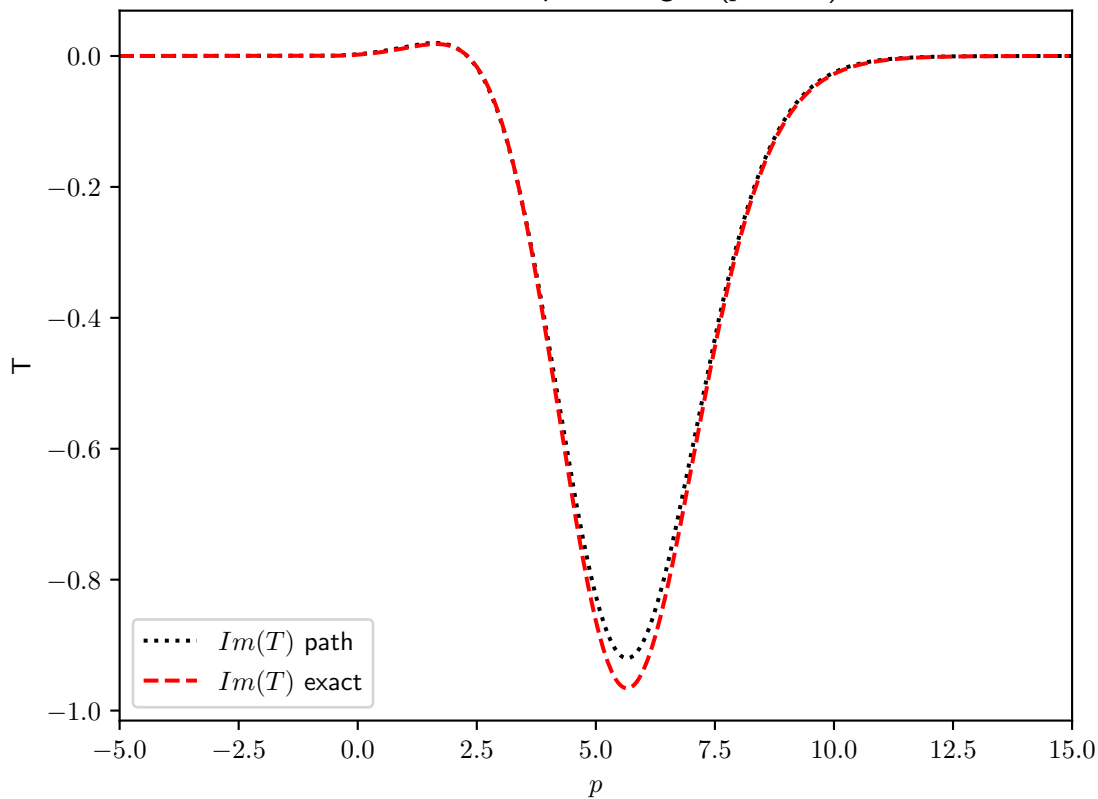
Im T exact vs path integral ( p = 5.0 )
