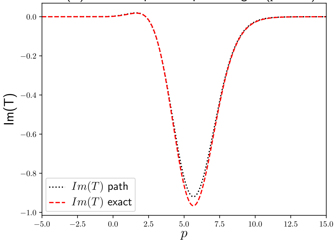
\text{Im}(T) exact compared to path integral ( p = 5.0 )
