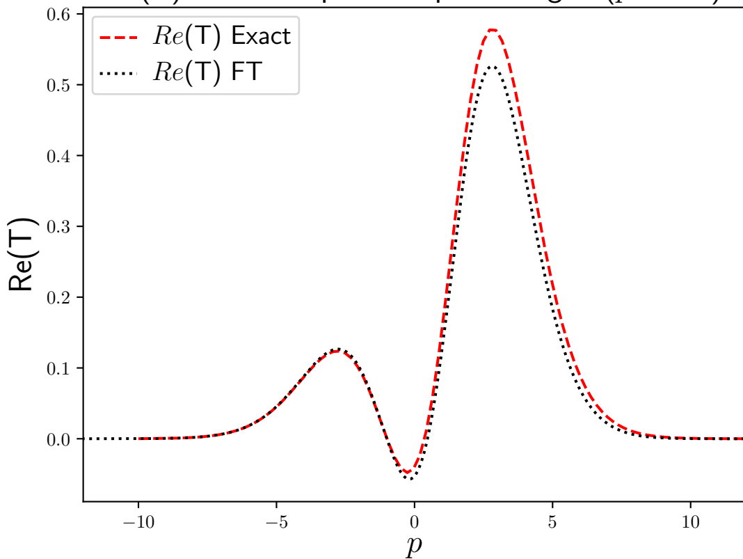
Re(T) exact compared to path integral ( p = 1.0 )
