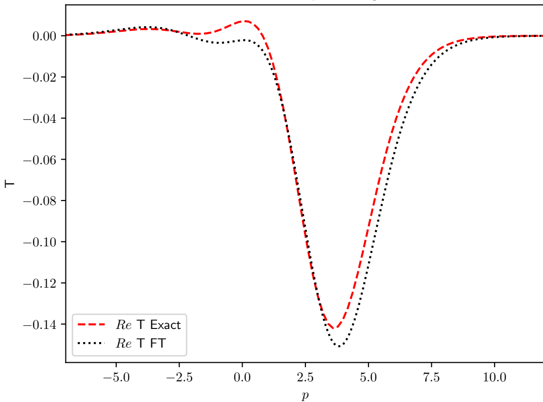
Re T exact vs path integral
