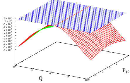
front form (BT-TP)/TP vs. Q , P_{12} ; Q perp to P_{12}
