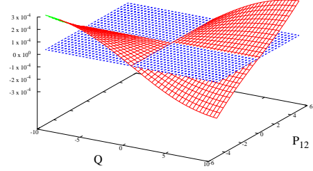
Figure 2: Front form - p_{12} \parallel Q
