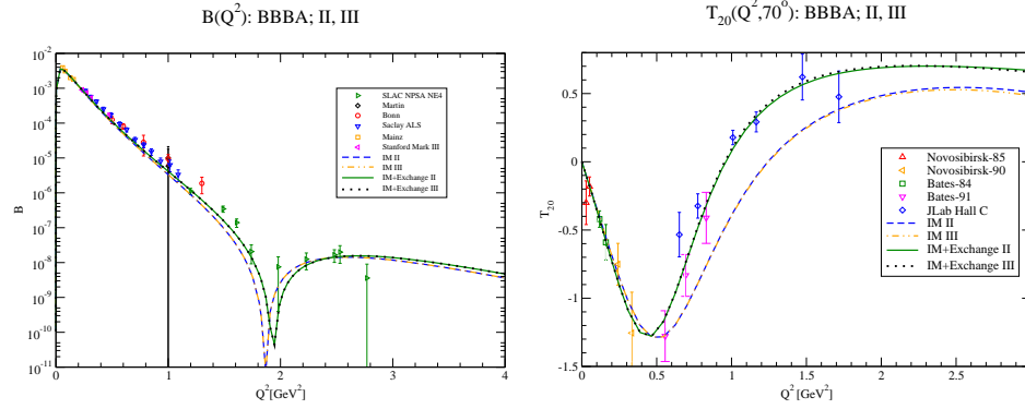
Fig. 5 Comparison of a front-form calculation of the elastic electron-deuteron tensor polarizable B(Q^2) with and without “pair current” contributions. Fig. 6 Comparison of a front-form calculation of the elastic electron-deuteron tensor polarizable T_{20}(Q^2, 70^\circ) with and without “pair current” contributions.
