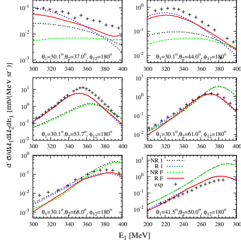
Fig. 2 Comparison of relativistic and non-relativistic calculations of exclusive proton deuteron breakup scattering at non-symmetric angles.
