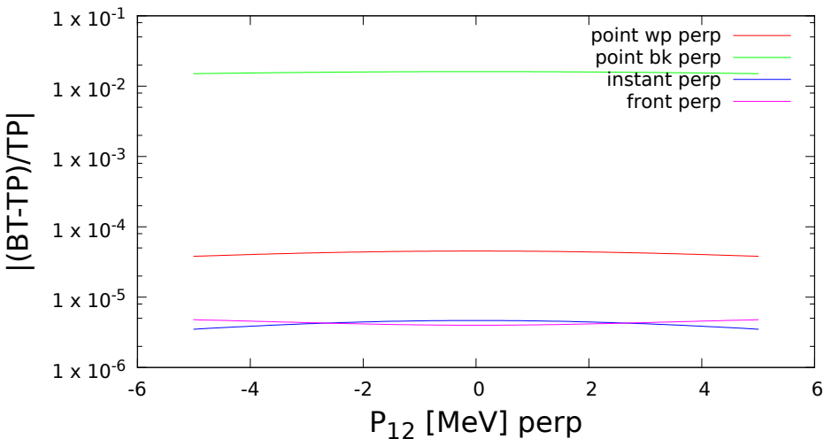
all forms - (BT-TP)/TP, q = 10 vs P_{12} perp
