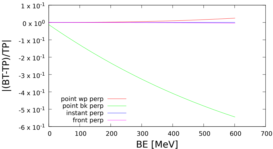
all forms - (BT-TP)/TP vs. BE, q = 10 , P_{12} perp=5
