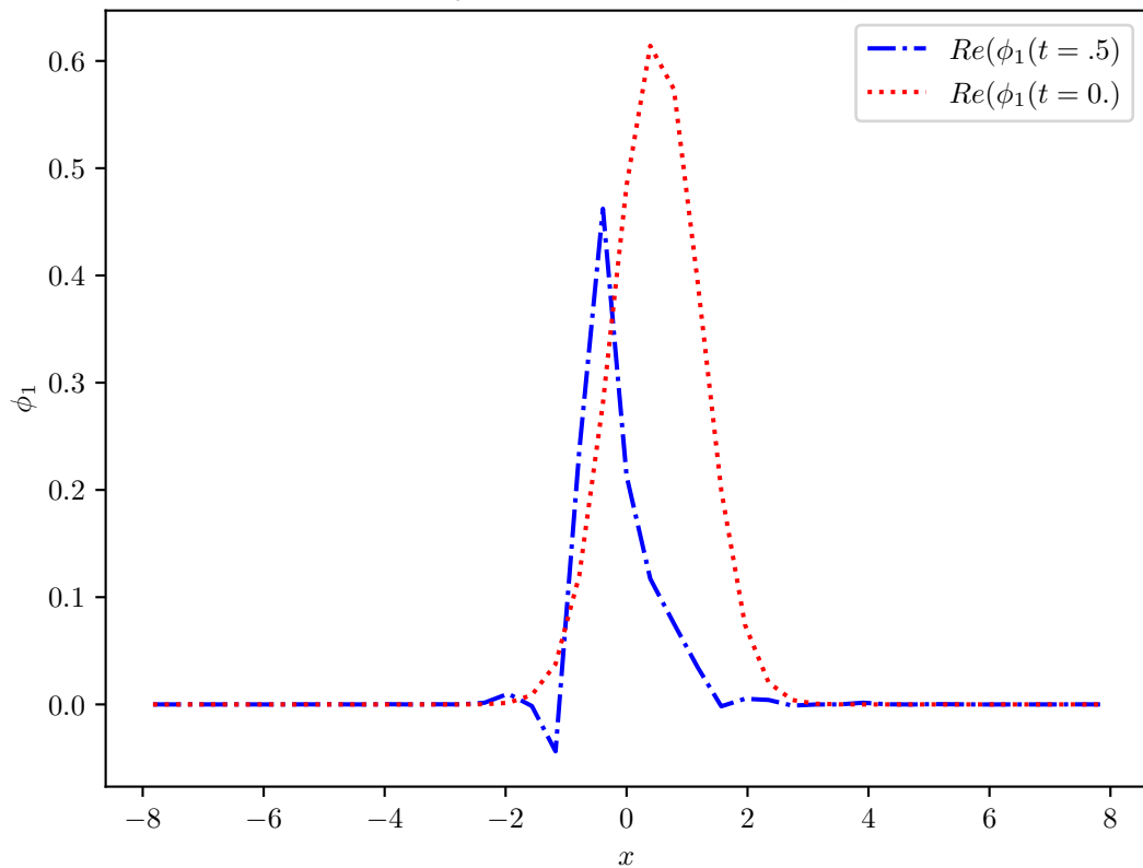
Real part of one mode at T = 0, .5
