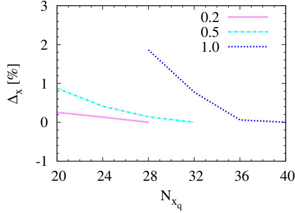
FIG. 2: (Color online) The percent error \Delta_x = \frac{\sigma_{op} - \sigma_{tot}}{\sigma_{op}} \times 100 in the optical theorem as function of the grid points in the angle grid x_q , when this grid is increased successively by 4 Gauss-Legendre points. The different curves correspond to the three different laboratory projectile energies in GeV, indicated in the legend.
