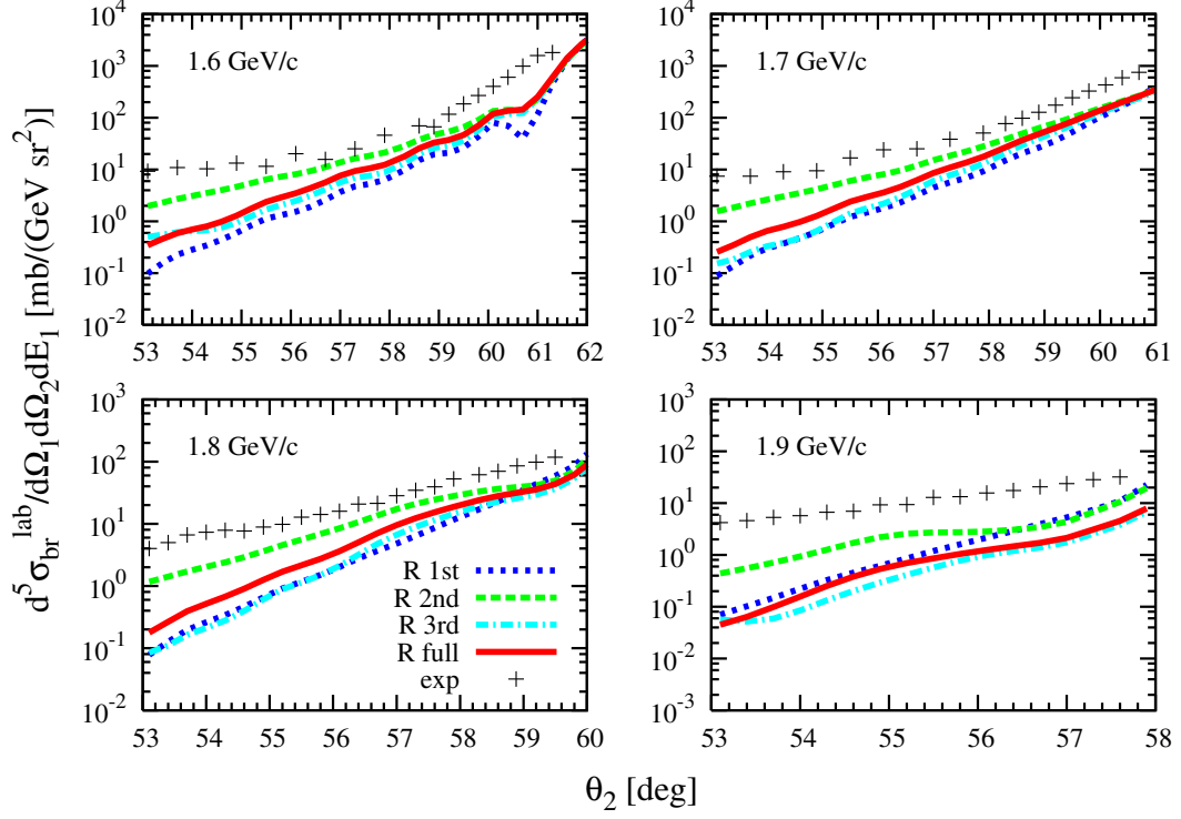
FIG. 13: (Color online) The exclusive differential cross section for the reaction ^1\text{H}(d,2p)n at 2 GeV deuteron energy as function of the angle \theta_2 of the second of the outgoing protons for a fixed first proton momentum indicated in the figure. The solid line represents the solution of the full relativistic Faddeev equation. The dotted line gives the result of the first order calculation. For the dashed line the 2nd order term is added and for the dash-dotted line the 2nd and 3rd order terms are added. The data are taken from Ref. [33].
