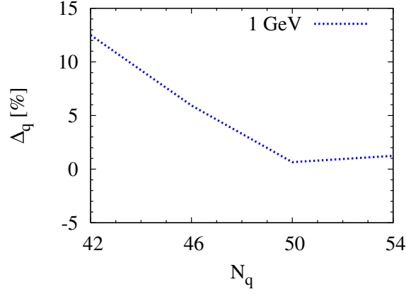
FIG. 1: (Color online) The percent error \Delta_q = \frac{\sigma_{op} - \sigma_{tot}}{\sigma_{op}} \times 100 in the optical theorem as function of the grid points in the momentum q for a calculation at 1.0 GeV.
