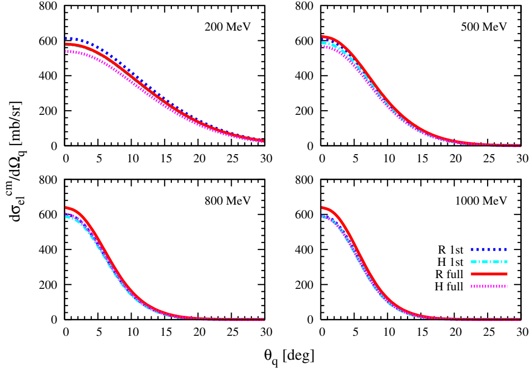
FIG. 6: (Color online) The differential cross section for elastic scattering as function of c.m. angle \theta_q for selected laboratory kinetic energies. The converged solution of the relativistic Faddeev equation is given as solid line. The dotted line shows the converged solution of the relativistic Faddeev equation in which the fully off-shell 2N t-matrix is replaced by the half-shell t-matrix. The corresponding first order calculation are given by the short-dashed line and the dash-dotted line. For details see text.
