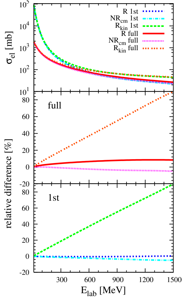
FIG. 5: (Color online) The total cross section for elastic scattering as function of the projectile kinetic energy (top panel). The fully relativistic Faddeev calculation is shown as solid line, the corresponding first order term by the short dashed line. Calculations which only use relativistic kinematics, i.e. the Lorentz transformation between laboratory and c.m. frame together with the relativistic phase space factor (labeled R_{\text{kin}} ) are given as dotted line for a full Faddeev calculation and as short-dashed line for the first order term. Calculations which only take into account the Lorentz transformations between the laboratory and c.m. frame (labeled \text{NR}_{\text{c.m.}} ) are shown as dotted line for the full Faddeev calculation and as dash-dotted line for the 1st order one. The middle panel shows the relative difference between the fully relativistic Faddeev calculation and the nonrelativistic one (solid line) together with the difference to the nonrelativistic calculation if only relativistic kinematics is considered. The bottom panel shows the corresponding relative differences when only the first order term is taken into account.
