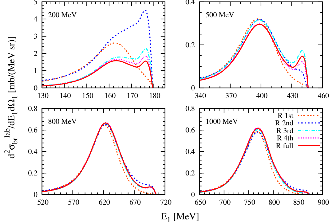
FIG. 10: (Color online) The inclusive breakup cross section as function of the laboratory kinetic energy E_1 of the emitted particle at an emission angle \theta_1 = 24^\circ . The incident laboratory kinetic energy for each cross section is indicated in each panel. The solid lines (R) represent the converged relativistic Faddeev calculation. The triple-dotted line shows the 1st order calculation, for the short dashed line the 2nd order contribution is added to the previous, for the dash-dotted line the 3rd order is added, and for the dotted line the 4th order.
