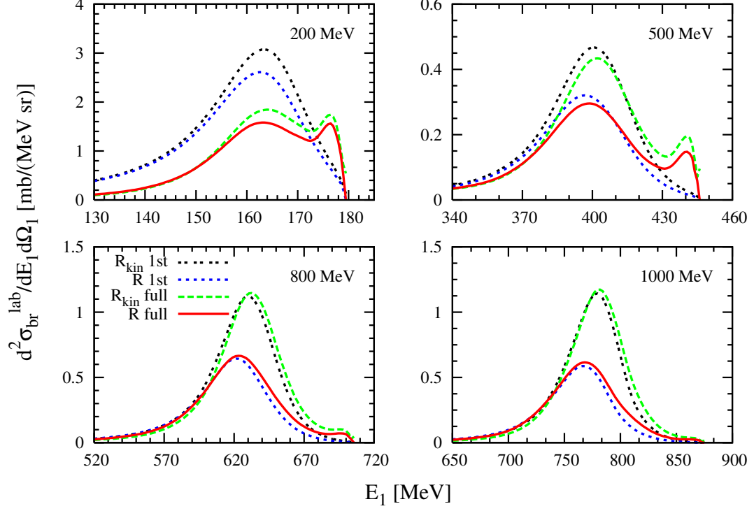
FIG. 9: (Color online) The inclusive breakup cross section as function of the laboratory kinetic energy E_1 of the emitted particle at an emission angle \theta_1 = 24^\circ . The incident laboratory kinetic energy for each cross section is indicated in each panel. The solid lines (R full) represent the converged relativistic Faddeev calculation and the dotted line the corresponding first order calculations (R 1st). The lines labeled R_{\text{kin}} correspond to calculations in which only relativistic kinematics is taken into account.
