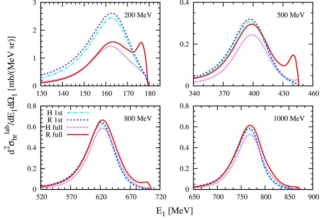
FIG. 11: (Color online) The inclusive breakup cross section as function of the laboratory kinetic energy E_1 of the emitted particle at an emission angle \theta_1 = 24^\circ . The incident laboratory kinetic energy for each cross section is indicated in each panel. The solid lines (R) represent the converged relativistic Faddeev calculation. The dotted line (H) displays the calculation in which the fully off-shell two-body t-matrix is replaced by the half-shell one. The calculations labeled 1st stand for the corresponding 1st order calculations.
