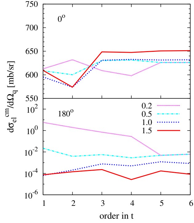
FIG. 8: (Color online) The differential cross section for elastic scattering in forward ( 0^\circ ) and backward ( 180^\circ ) direction as function of the order in the multiple scattering series for selected projectile laboratory kinetic energies indicated in the legend in units of GeV.
