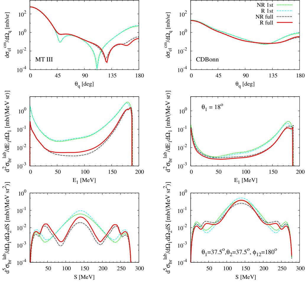
FIG. 4: (Color online) Three nucleon scattering at laboratory projectile kinetic energy E_{lab} = 200 MeV. The left column shows results obtained from the Malfiet-Tjon-III potential assuming boson symmetry and no partial wave decomposition, the right column shows the corresponding realistic calculations obtained with the CD-Bonn [14] potential where partial wave decomposition is applied. The top row displays the differential cross section for elastic scattering, the middle row shows the breakup cross section for inclusive scattering for the laboratory angle \theta_1 = 18^\circ of the outgoing particle. The bottom row shows the five-fold differential for exclusive breakup reaction as function of the arc-length S . The laboratory angles of the outgoing particles are \theta_1 = \theta_2 = 37^\circ , and \phi_{12} = 180^\circ . The fully relativistic converged Faddeev calculations are given by the solid lines (R), the corresponding nonrelativistic calculations by the long-dashed lines (NR). In addition the relativistic (dash-dot) and nonrelativistic (dotted) first order calculations are shown.
