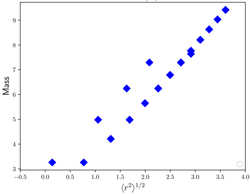
Mass versus \langle r^2 \rangle^{1/2}
