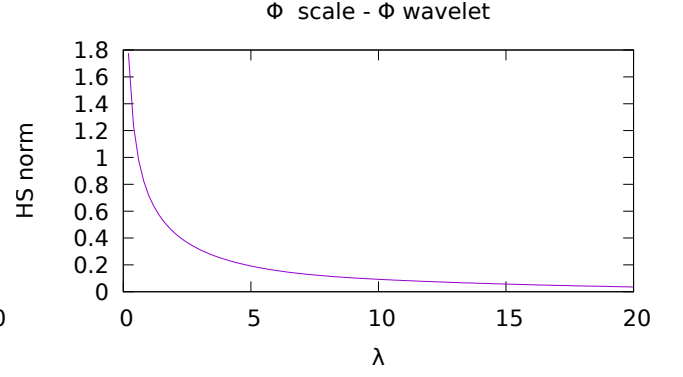
FIG. 4: Hilbert-Schmidt norm: \Phi scale - \Phi wavelet
