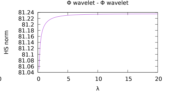
FIG. 2: Hilbert-Schmidt norm: \Phi wavelet - \Phi wavelet
