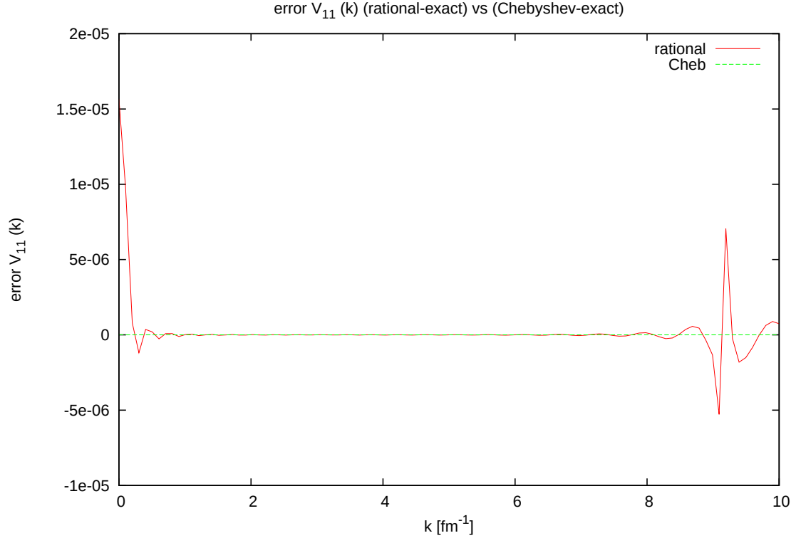
FIG. 13: \Delta V_{11\text{rational}}(k) , \Delta V_{11\text{Chebyshev}}(k) .
