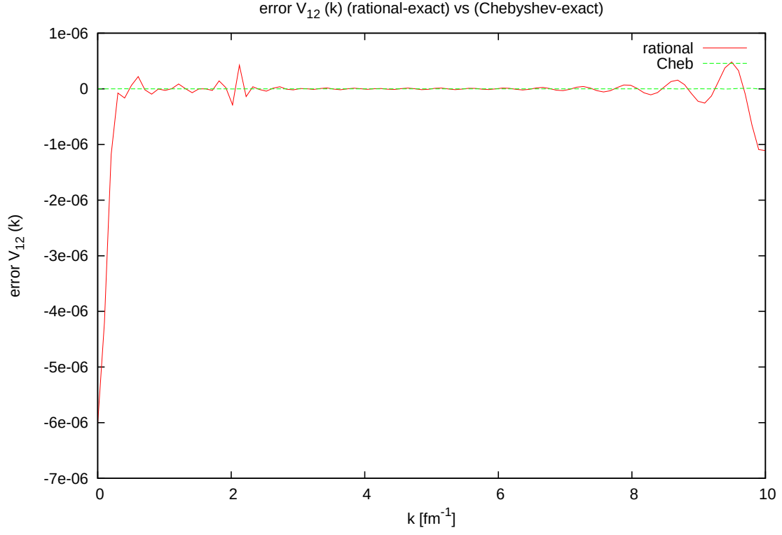
FIG. 14: \Delta V_{12\text{rational}}(k) , \Delta V_{12\text{Chebyshev}}(k) .
