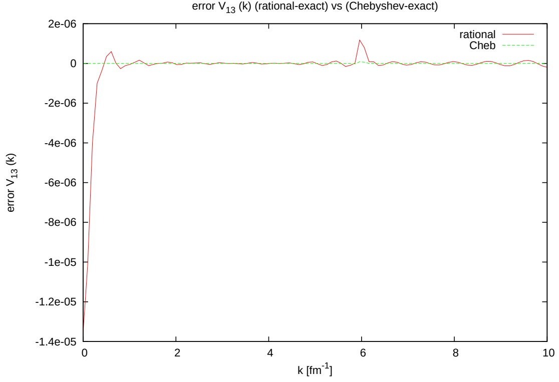
FIG. 15: \Delta V_{13\text{rational}}(k) , \Delta V_{13\text{Chebyshev}}(k) .
