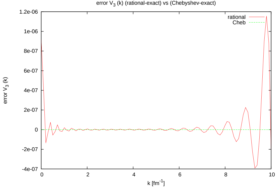
FIG. 5: \Delta V_{3 \text{ rational}}(k) , \Delta V_{3 \text{ Chebyshev}}(k) .
