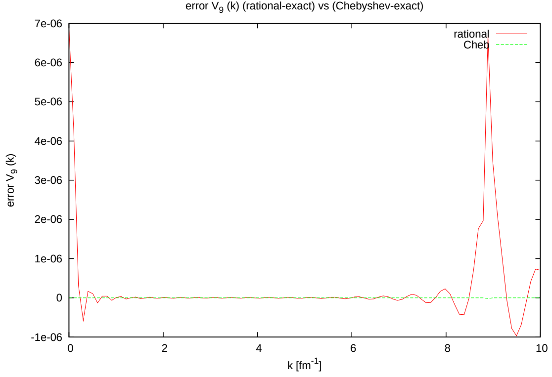
FIG. 11: \Delta V_{9brational}(k) , \Delta V_{9bChebyshev}(k) .
