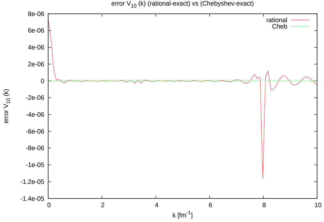
FIG. 12: \Delta V_{10\text{rational}}(k) , \Delta V_{10\text{Chebyshev}}(k) .
