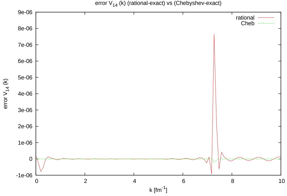
FIG. 16: \Delta V_{14\text{rational}}(k) , \Delta V_{14\text{Chebyshev}}(k) .
