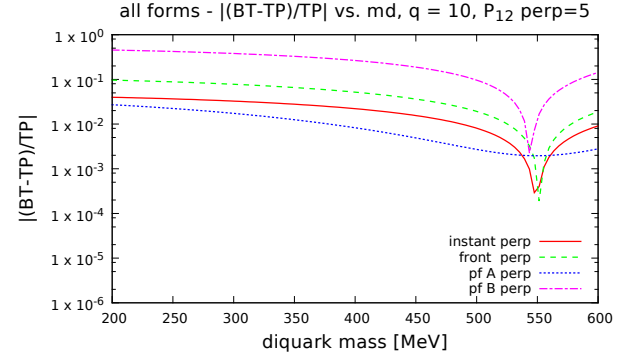
FIG. 15: (Color online) Model differences for BT calculations as a function of two-body spectator mass, \mathbf{q} = 10 \text{ fm}^{-1} \perp \mathbf{p}_{12} .
