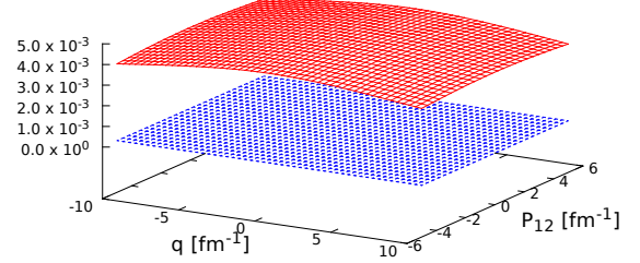
front form (BT-TP)/TP vs. q , P_{12} ; q perp to P_{12}
