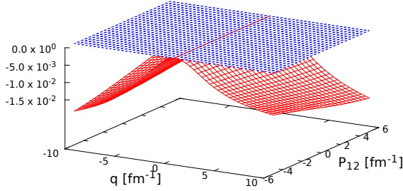
point form - B - (BT-TP)/TP vs. q , P_{12} ; q parallel to P_{12}
