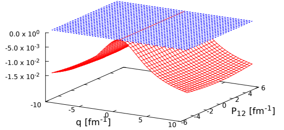
point form - B - (BT-TP)/TP vs. q , P_{12} ; q perp to P_{12}
