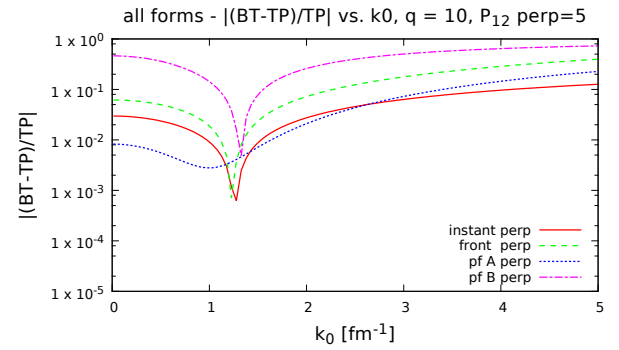
FIG. 17: (Color online) Model differences for BT calculations as a function of Gaussian wave function scale, \mathbf{q} = 10 \text{ fm}^{-1} \perp \mathbf{p}_{12} .
