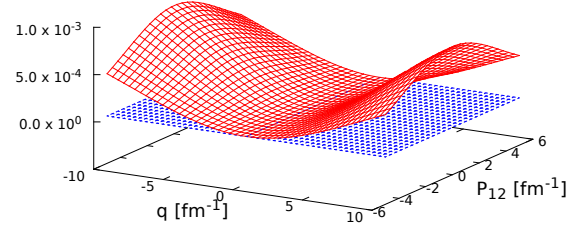
FIG. 3: (Color online) Model differences for instant-form BT calculation, \mathbf{q} \perp \mathbf{p}_{12} .
