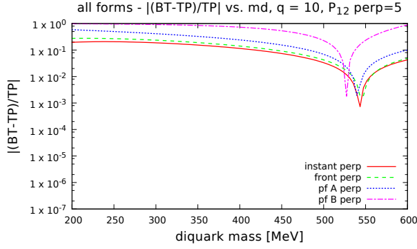
FIG. 14: (Color online) Model differences for BT calculations as a function of two-body spectator mass, \mathbf{q} = 10 \text{ fm}^{-1} \perp \mathbf{p}_{12} .
