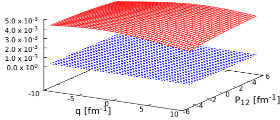
front form (BT-TP)/TP vs. q , P_{12} ; q parallel to P_{12}
