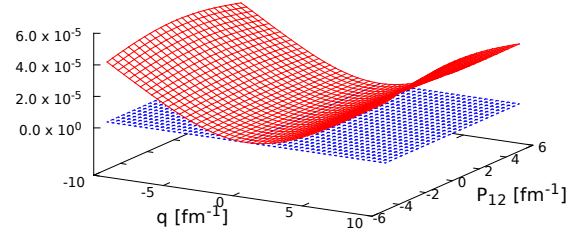
point form - A - (BT-TP)/TP vs. q , P_{12} ; q perp to P_{12}
