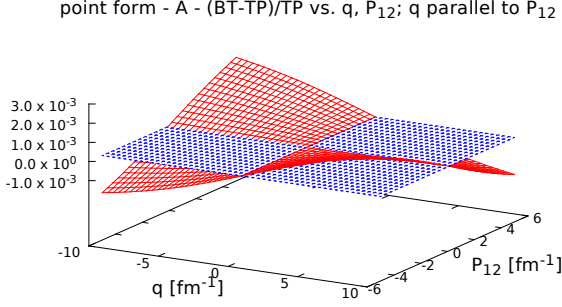
FIG. 6: (Color online) Model differences for point-form BT calculation A, \mathbf{q} \parallel \mathbf{p}_{12} .
