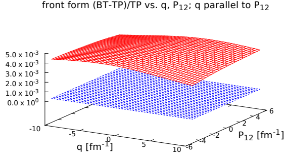
FIG. 4: (Color online) Model differences for front-form BT calculation, \mathbf{q} \parallel \mathbf{p}_{12} .
