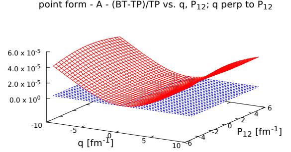
FIG. 7: (Color online) Model differences for point-form BT calculation A, \mathbf{q} \perp \mathbf{p}_{12} .
