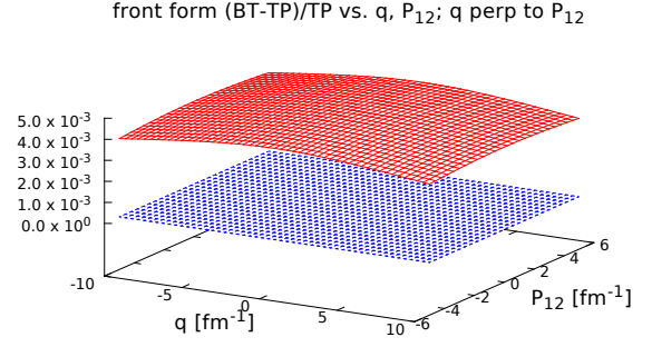
FIG. 5: (Color online) Model differences for front-form BT calculation, \mathbf{q} \perp \mathbf{p}_{12} .
