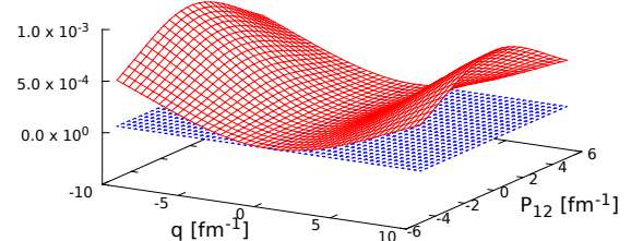
FIG. 3: (Color online) Model differences for instant-form BT calculation, \mathbf{q} \perp \mathbf{p}_{12} .
