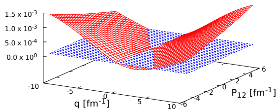
FIG. 2: (Color online) Model differences for instant-form BT calculation, \mathbf{q} \parallel \mathbf{p}_{12} .
