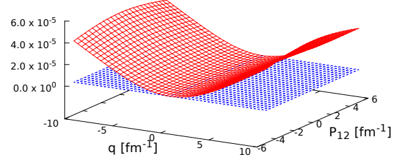
point form - (BT-TP)/TP vs. q , P_{12} ; q perp to P_{12}
