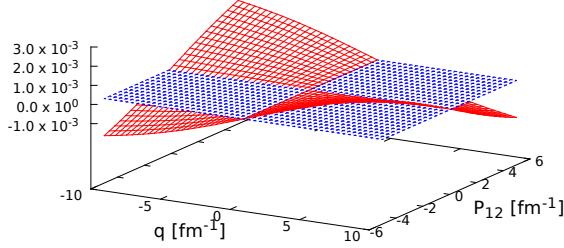
point form - (BT-TP)/TP vs. q , P_{12} ; q parallel to P_{12}
