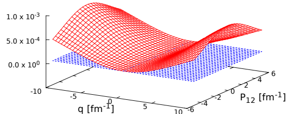
FIG. 3: (Color online) Model differences for instant-form BT calculation, \mathbf{q} \perp \mathbf{p}_{12} .
