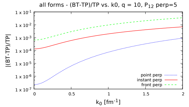
FIG. 11: (Color online) Model differences for BT calculations as a function of two-body Gaussian wave function scale, \mathbf{q} = 10 \text{ fm}^{-1} \perp \mathbf{p}_{12} .
